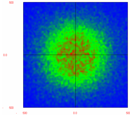
Raytrace Simulation of Typical Beam at 1m with 7 x 1W White LED's
