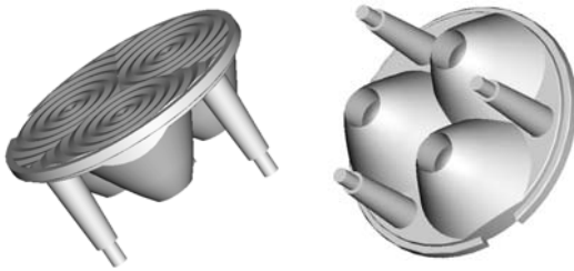
MR16/GU10 Light Fitting Optic
