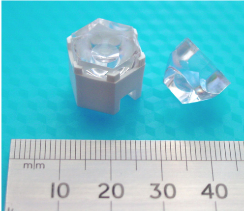
Small 12.9mm AF hexagon optic format in 15.2mm AF Holder enables optics to be close-packed in arrays
