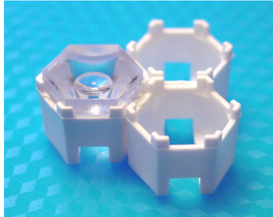
Small 12.9mm AF hexagon optic format in 15.2mm AF Holder enables optics to be close-packed in arrays
