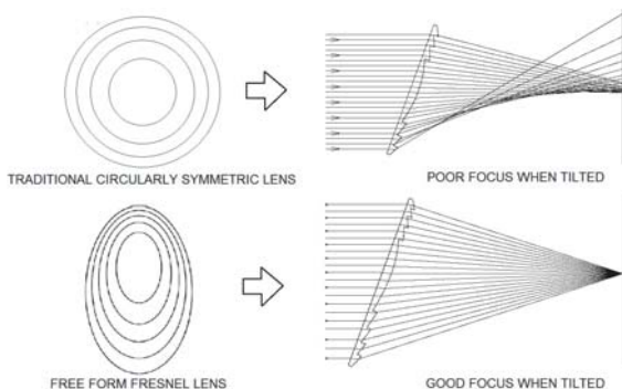
Diagram shows theory behind free-form lens design
